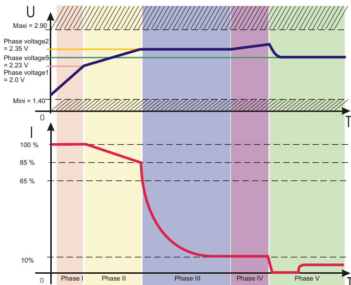
5 states charging curve
